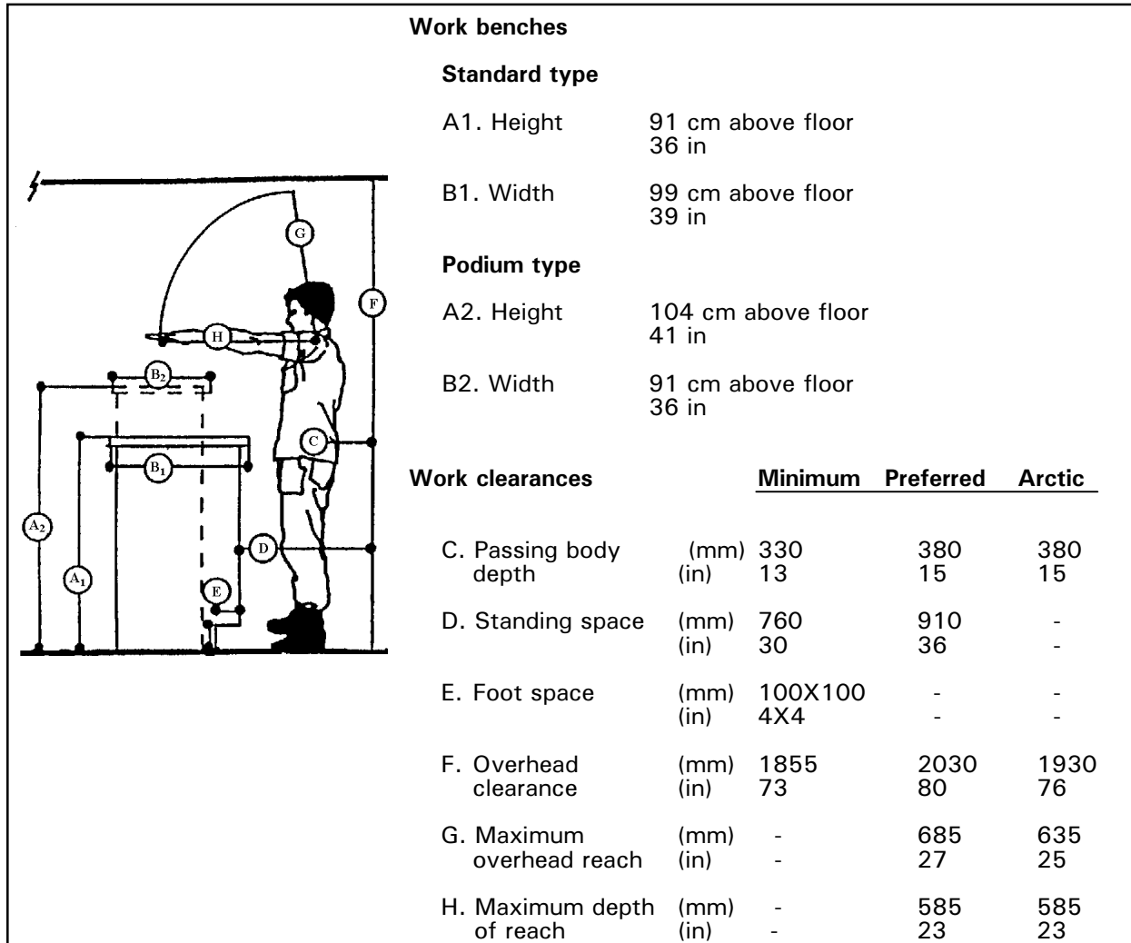
Exhibit 9.4.3.1 Standing workplace illustration and dimensions
