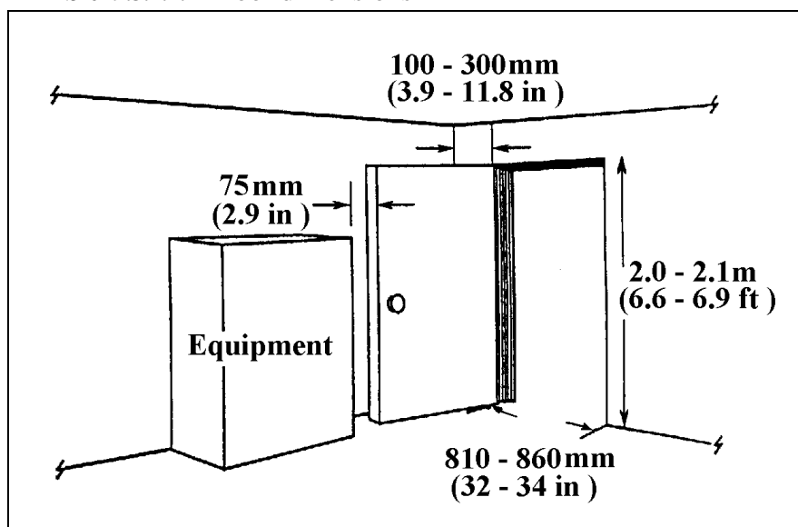
Exhibit 9.3.4.2.1 Door dimensions
