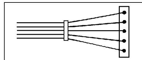
Exhibit 6.14.2.13 Terminal strips
