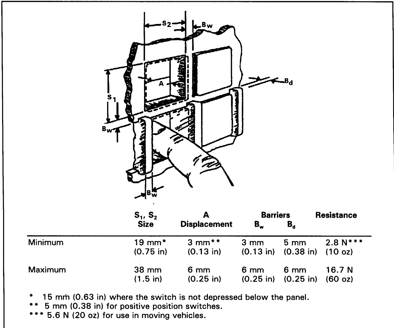
Exhibit 7.4.4.11.1 Legend switch specifications
