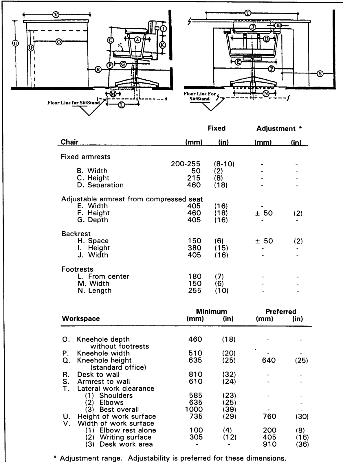
Exhibit 9.4.4.4 Seated workspace dimensions and illustrations
