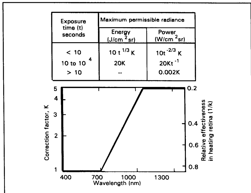
Exhibit 12.14.3.1 Maximum safe exposure to 400-1400 nm radiant energy
