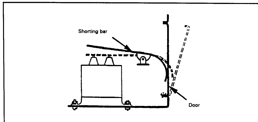
Exhibit 12.4.3.3 Automatic shorting bar
