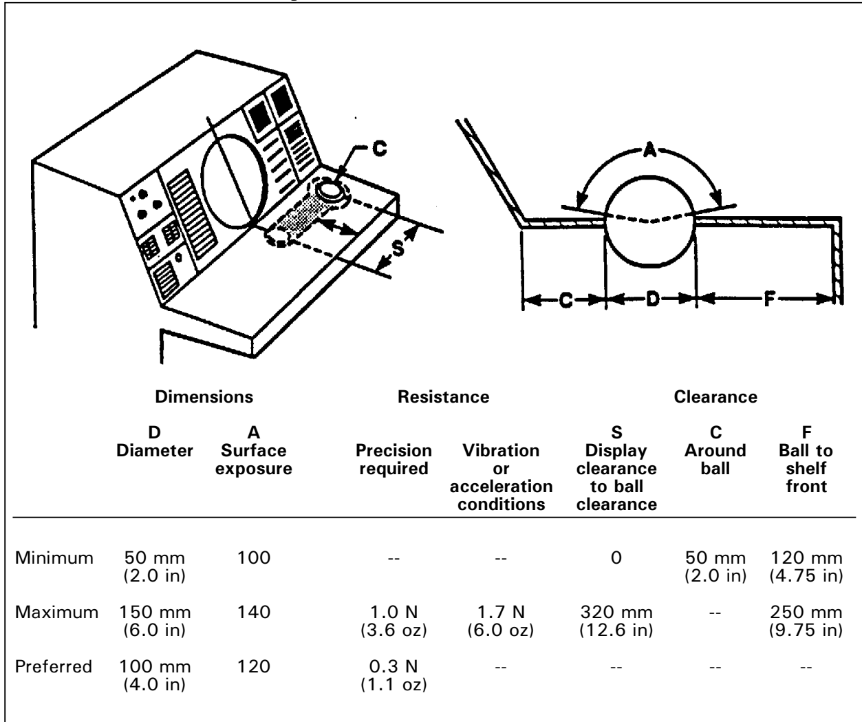
Exhibit 7.4.4.22.1 Ball control specifications
