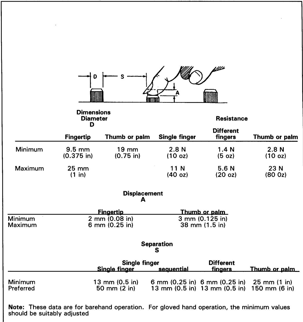
Exhibit 7.4.4.8.1 Push button specifications
