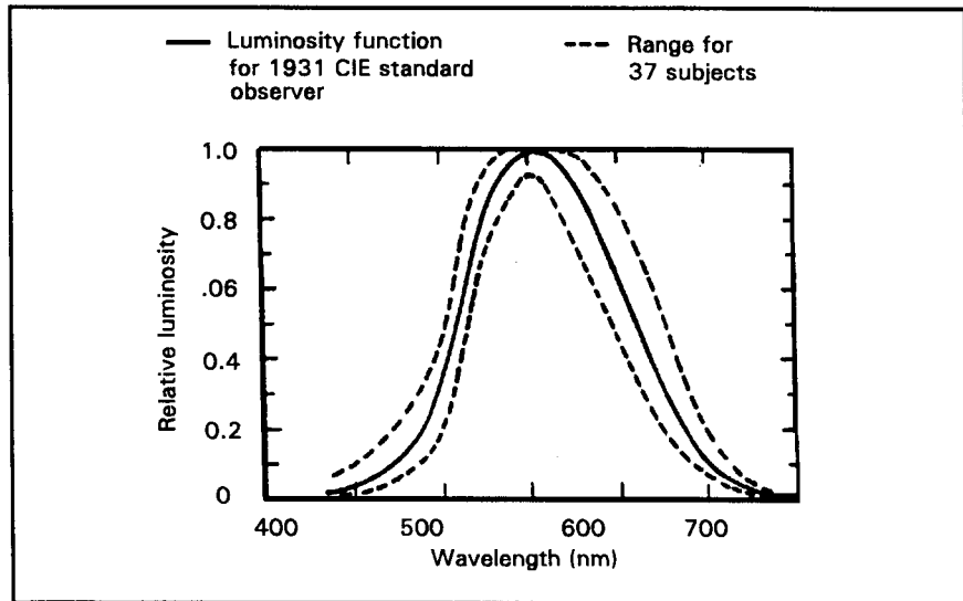
Exhibit 12.14.3 Relative contribution of different wavelengths to luminance--the luminosity function
