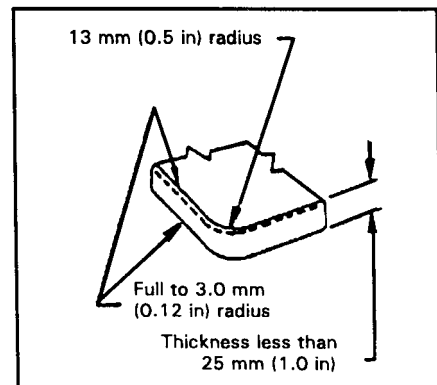
Exhibit 12.5.1.5 (a) Requirements for rounding of corners less than 25 mm (1.0 in) thick
