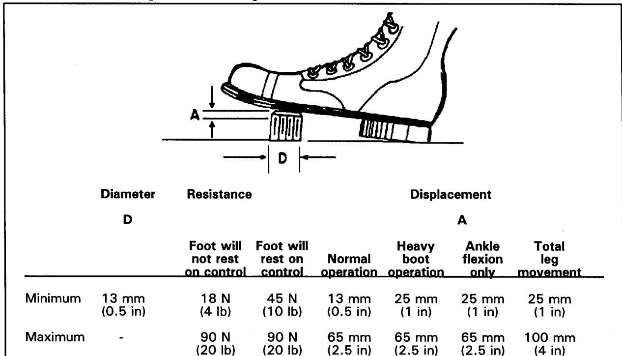
Exhibit 7.4.3.1 Foot-operated switch specifications
